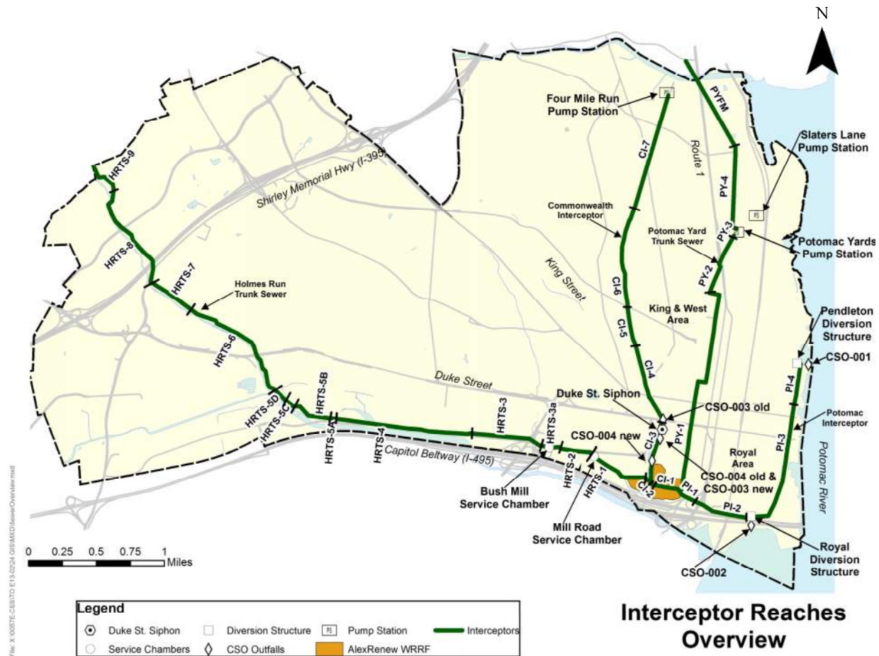
Figure 8-1: AlexRenew Interceptor System Overview
