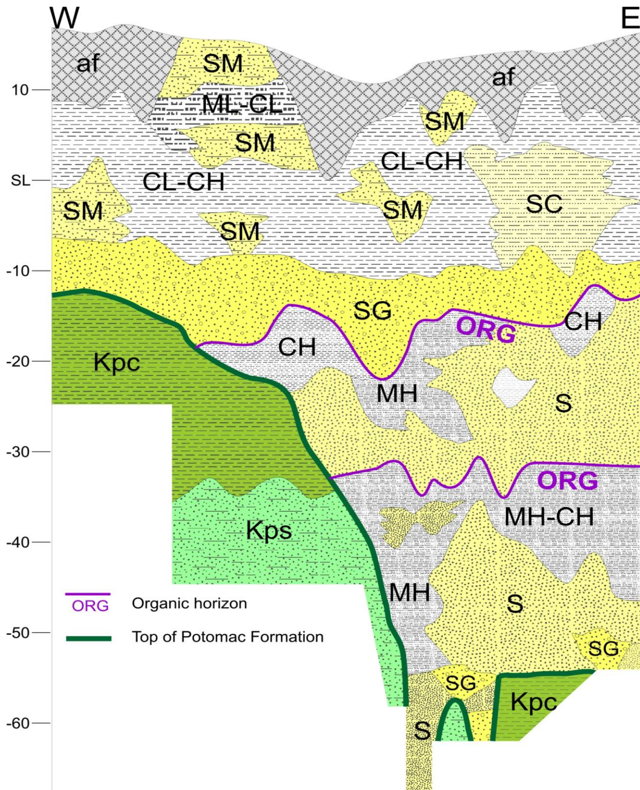
Figure 5-21. Subsurface interpretation of geotechnical boring site 117 in the northern part of the Old Town terrace (see plate 1 for location). The site is about 1,200 feet wide, with dozens of deep borings. Units are: Kps, Kpc-sand and clay of the Potomac Formation; SG-sand and gravel; S-medium-coarse sand; SM-silty sand; SC-clayey sand; CH, MH-plastic clay and silt; CL, ML-non-plastic clay and silt; af-artificial fill. The sharp east-facing escarpment on the top of the Potomac Formation appears to bound the thalweg of the late Pleistocene Potomac River.
