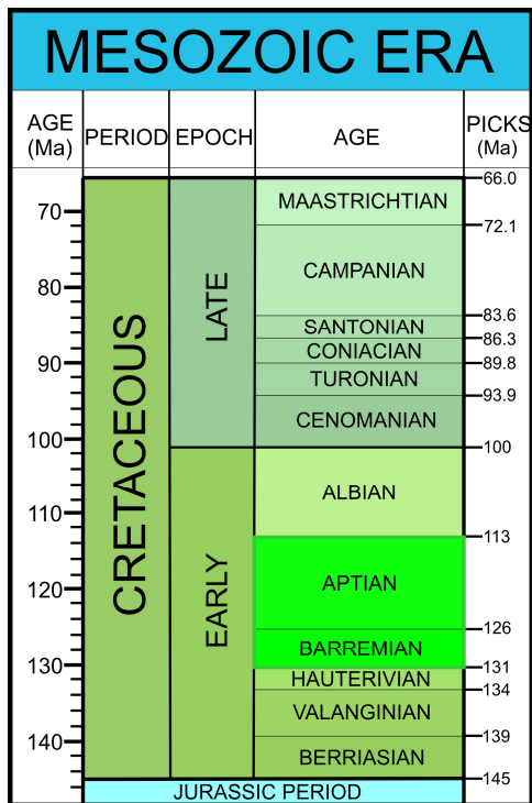
Figure 4-3. Left: Detailed geologic time scale of the Cretaceous Period. The microfossil age of the Potomac Formation in the map area is highlighted in bright green. Ages and picks from the Geological Society of America (2012). Right: Rendering of an early Cretaceous backswamp similar to those represented by some of the Potomac Formation units on plate 4. Courtesy of the Smithsonian Institution.
