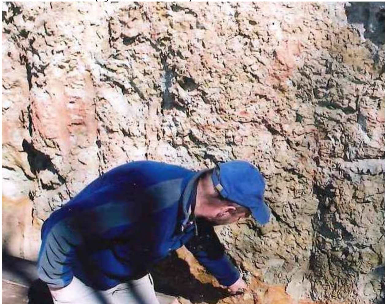
Figure 4-26. Greenish-gray, fractured clay with reddish mottled areas above, at the type locality on Arell Court. Many fracture surfaces are slickensided. Photo by Rod Simmons.
