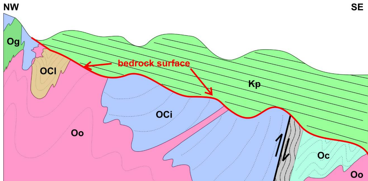
Figure 3-1. Schematic diagram illustrating the angular unconformity represented by the bedrock surface beneath the map area. The Piedmont bedrock (represented by units OCI, Oci, Oc, Og, Oo) was complexly folded, faulted, metamorphosed, and raised into a large mountain range before being beveled by erosion to a low-relief surface. The overlying Potomac Formation (Kp) was deposited along the erosion surface and, other than being gently tilted to the southeast and locally faulted, is essentially undeformed. Note also that the unconformity represents a hiatus of more than 300 million years in the local geologic record, between the Ordovician bedrock (circa 460-475 ma) and the overlying Cretaceous strata (circa 130 ma). Not to scale.
