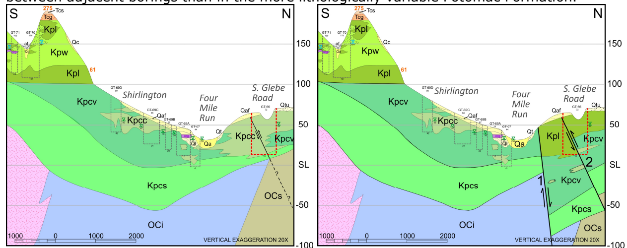
Figure 8-18. Cross sections illustrating competing explanations of the geologic structure in the vicinity of Shirley Highway and Four Mile Run. In one interpretation (left), the large body of clayey silt on the north side of Four Mile Run (Kpcc) and the sands to the south (Kpcv) are in a lateral facies relationship: the silt is considered to be a fine-grained sedimentary facies deposited in a backswamp localized along the north margin of the Four Mile Run bedrock valley, whereas the thick sand units are developed over the thalweg of the bedrock valley. The "small fault seen in outcrop" by Drake et al (1979) is just that, with negligible offset of strata. In an alternate interpretation (right), the thick plug of silt represents a downthrown block of Lincolnia silty clay (Kpl)—a map unit prominent in the bluffs just to the south and west—which has been juxtaposed against stratigraphically lower sands (Kpcv) along a normal fault (1). In this model, the fault (2) mapped by Drake and others (1979) assumes greater importance and is responsible for the seemingly abrupt change from silt to sand in the lower part of the borings in the northern part of the S. Glebe Road interchange (GT-66, highlighted by the red dashed line), resulting in a small, graben-like structure between the two faults. In the absence of more definitive evidence, however, no major fault is currently postulated at this location, and the structural relations depicted on the maps and cross sections are as shown in the left hand diagram.
