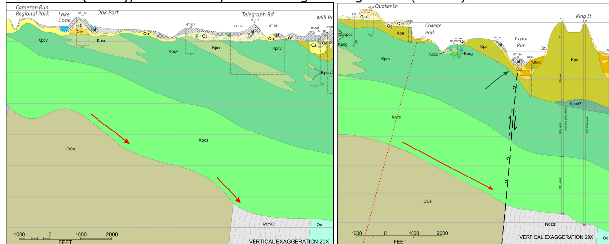
Figure 8-19. Left: In the Eisenhower Valley, the slope of the bedrock surface appears to steepen (arrows) between Oak Park and Telegraph Road as the west wall of the RCSZ is approached. This feature coincides with an exceptionally thick section of the Cameron Valley sand member (Kpcs-Kpcv-Kpcc) — 250 to 300 feet — greater than anywhere else in the map area. Right: Further north, along Duke Street, the increased gradient of the bedrock surface (red arrow) and sharp changes in the thickness and base elevation of the Arell clay member (Kpa; green arrow) suggest the presence of a flexure (red dashed line) and fault zone in the Potomac Formation (queried black dashed line). Light gray horizontal lines are 50-foot elevation reference lines.
