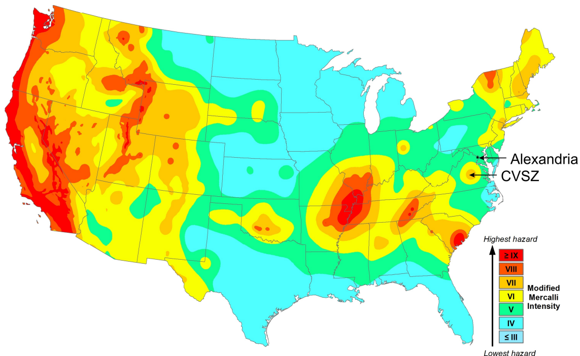
Figure 8-6. USGS map showing the intensity of potential earthquake ground shaking that has a 2% chance of occurring in 50 years. CVSZ-Central Virginia Seismic Zone. Source: http://gallery.usgs.gov/images/wordpress/20150810/GroundShaking.jpg
