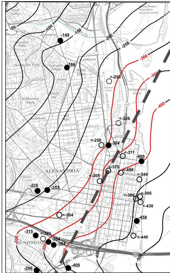
Figure 8-20. Bedrock topography in the eastern part of the map area. Contour interval is 50 feet. Solid circles and numbers are firm bedrock elevations reported in wells that reached the bedrock surface. Open circles and "less than" numbers represent the bottom elevations of wells that did not reach the bedrock surface. The bedrock surface slope increases across a north to northeast trending zone indicated by the red contours. The steepest part of the structure appears to underlie the northwestern part of Old Town, where the contours are most tightly spaced, however, that could be an artifact of greater data density than elsewhere along the structure. The heavy dashed line marks the trend of a hypothetical fault.
