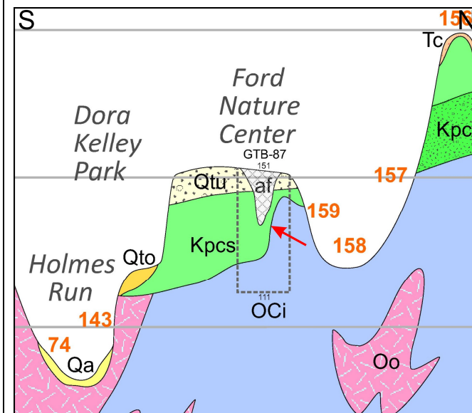
Figure 8-12. Part of the Van Dorn St. cross section (plate 2I) illustrating the sharp bedrock surface slope (red arrow) beneath Ramsay Elementary School/Ford Nature Center (site GTB-87). Light gray horizontal lines are 50-foot elevation reference lines. Orange numbers are outcrops shown on plate 1. Geologic units are: af – artificial fill; Qa – modern alluvium; Qtu, Qto – late Pleistocene stream terraces; Tc – colluvium; Kpcs, Kpcg – Potomac Formation, Cameron Valley sand member; Oo – Ocoquan granite; OCi – Indian Run Formation. Width of cross section: about 2,800 ft.
