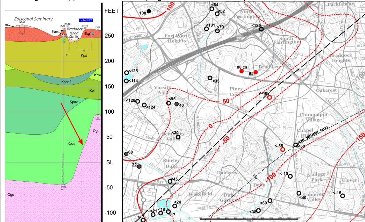
Figure 8-17. Left: The abrupt change in elevation of the bedrock surface below the seminary appears as an almost scarp-like face (arrow) at the north end of the Hospital cross section (H-H'). Geologic units are: Ogu – undifferentiated granitic bedrock; Kpcs, Kpcv, Kpl, Kpw, Kpch, Kpa – Potomac Formation; Tsg, Tsm – Seminary terrace. Right: An alternative interpretation of bedrock topography (dashed red lines) in the central part of the map area if the sharp slope on the bedrock surface below the seminary is interpreted as a dissected fault scarp. Compare to plate 3 . The hypothetical fault appears as a heavy dashed black line, roughly paralleling the Fort Williams fault. Solid dots and numbers are firm bedrock elevations at boreholes that reached the bedrock surface. Open circles and "less than" numbers represent the bottom elevations of boreholes that did not reach the bedrock surface. The well numbers mentioned in the text are shown in red.
