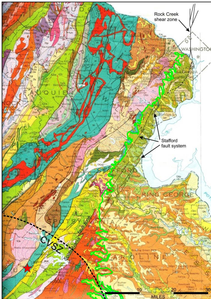
Figure 8-3. Portion of the Geologic Map of Virginia (Virginia Division of Mineral Resources, 1993) showing northeastern Virginia. The green line is the approximate location of the Fall Zone, separating the Piedmont to the west and the Coastal Plain to the east. Heavy dark lines are faults; faults that project into Alexandria are labeled. The red star near the southwest corner is the epicenter of the 2011 Mineral earthquake, while the dashed line is the approximate northern edge of the Central Virginia Seismic Zone (CVSZ; Horton and others, 2015, and references therein), a distinct area of moderate historical seismicity. The pronounced northeast-to-southwest orientation of geologic structures likely facilitates preferential transmission of seismic energy in the same direction (Hough, 2012), and may explain why the 2011 Mineral earthquake was felt so strongly in the Washington, DC area.
