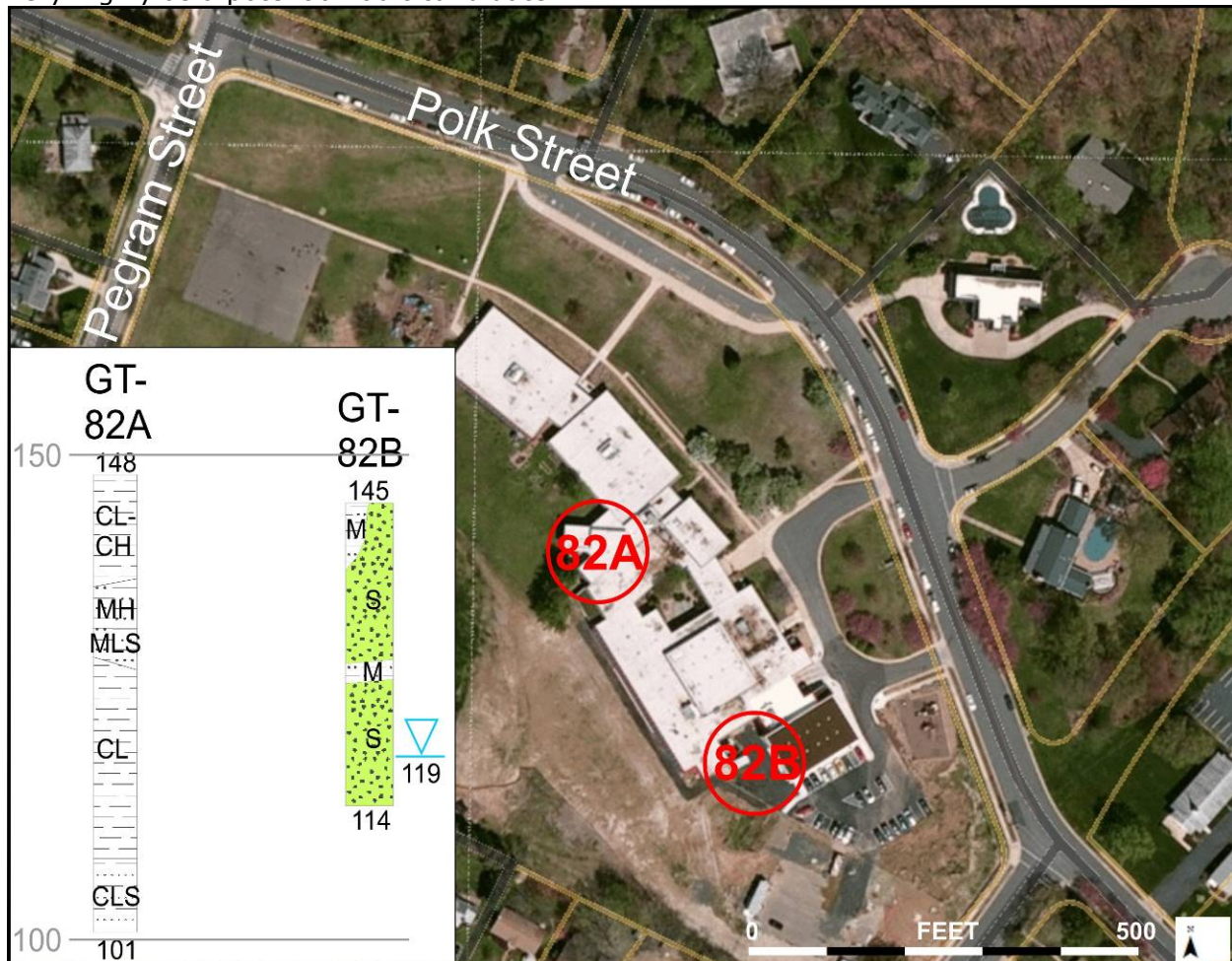
Figure 8-14. Aerial photograph of James Polk Elementary School (GTB #82) showing the locations of the two sets of geotechnical borings, which are illustrated by the schematic summary diagrams in the inset. Site 82A includes 4 borings for the library addition, all of which consisted entirely of variably sandy silts (MH, MLS) and silty clays (CL, CH, CLS) typical of the Lincolnia silty clay member of the Potomac Formation. Site 82B consists of three ground water monitoring wells at a former UST site, all of which penetrated dense, green-gray sand (S) with minor sandy silt layers (M), presumably the Cameron Valley sand member. Light gray horizontal lines are the 100 and 150-foot elevation reference lines. Numbers above and below the boring logs represent the maximum surface elevation and lowest elevation penetrated, respectively, in each set. Aerial photo from City of Alexandria parcel viewer
