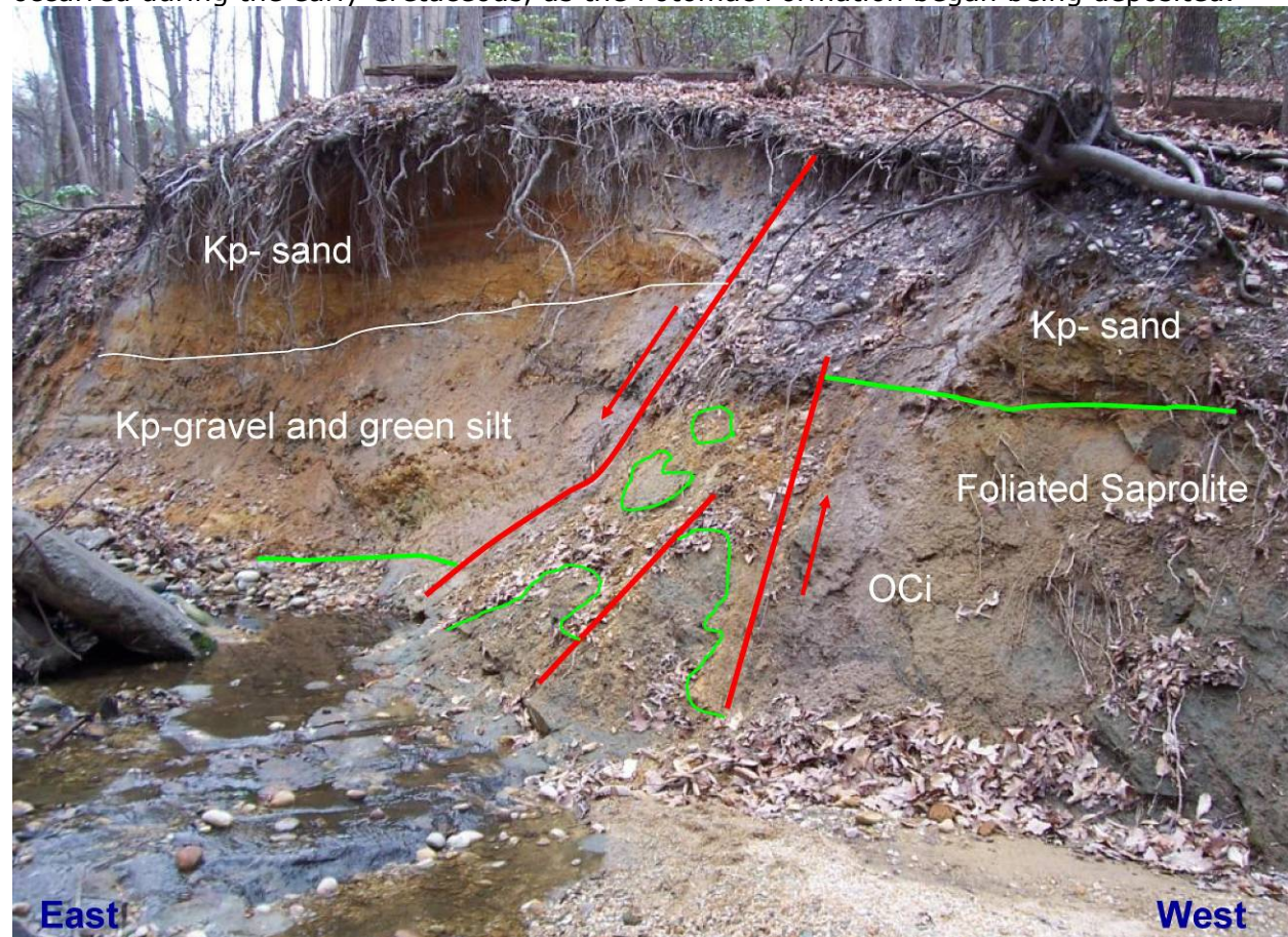
Figure 8-9. The Chambliss Park fault. Red lines and arrows denote fault walls and sense of motion, respectively. Heavy green line denotes bedrock surface on the Indian Run Formation (OCi). The base of the Potomac Formation (Kp) on the east side of the fault consists of coarse gravel interbedded with green silt, whereas it is sand on the west side. The zone in the middle appears to consist of blocks of bedrock (outlined in green) floating in Potomac Formation sand (Kp). West is to the right. The gravel at the top of the cut is colluvium. Photo by Tony Fleming.
