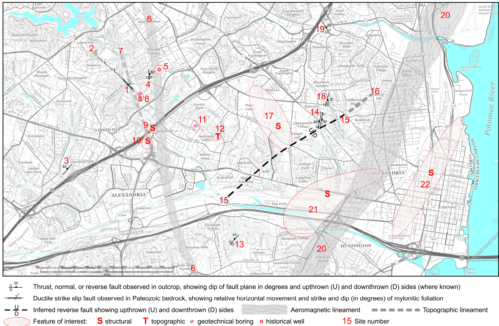
Figure 8-8. Index map of faults, lineaments, and other features of interest discussed in this section.
