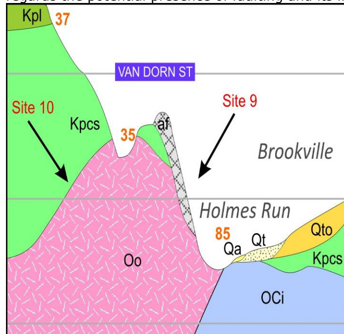
Figure 8-13. Part of the Shirley Highway cross section ( plate 2L ) illustrating the relatively steep bedrock surface slopes (arrows) at Brookville (site 9) and beneath Landmark (site 10). North is to the right. Light gray horizontal lines are 50-foot elevation reference lines. Orange numbers are outcrops. Geologic units are: af – artificial fill; Qa – modern alluvium; Qt, Qto – late Pleistocene stream terraces; Kpcs – Potomac Formation, Cameron Valley sand member; Kpl – Potomac Formation, Lincolnia silty clay member; Oo – Occoquon granite; OCi – Indian Run Formation. Width of cross section: about 3,300 ft.
