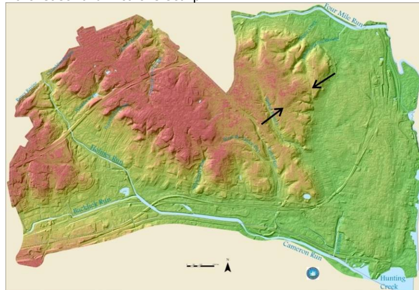
Figure 8-16. Topographic lineament (between arrows) parallel to the Jefferson Park escarpment is prominent on the Alexandria DEM.
