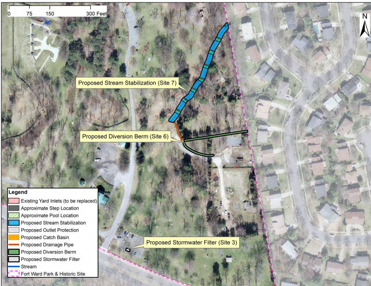
Figure D-4: Proposed Concept Design Location
