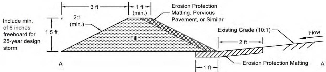
Figure D-5: Proposed Diversion Berm Concept Design Cross Section
