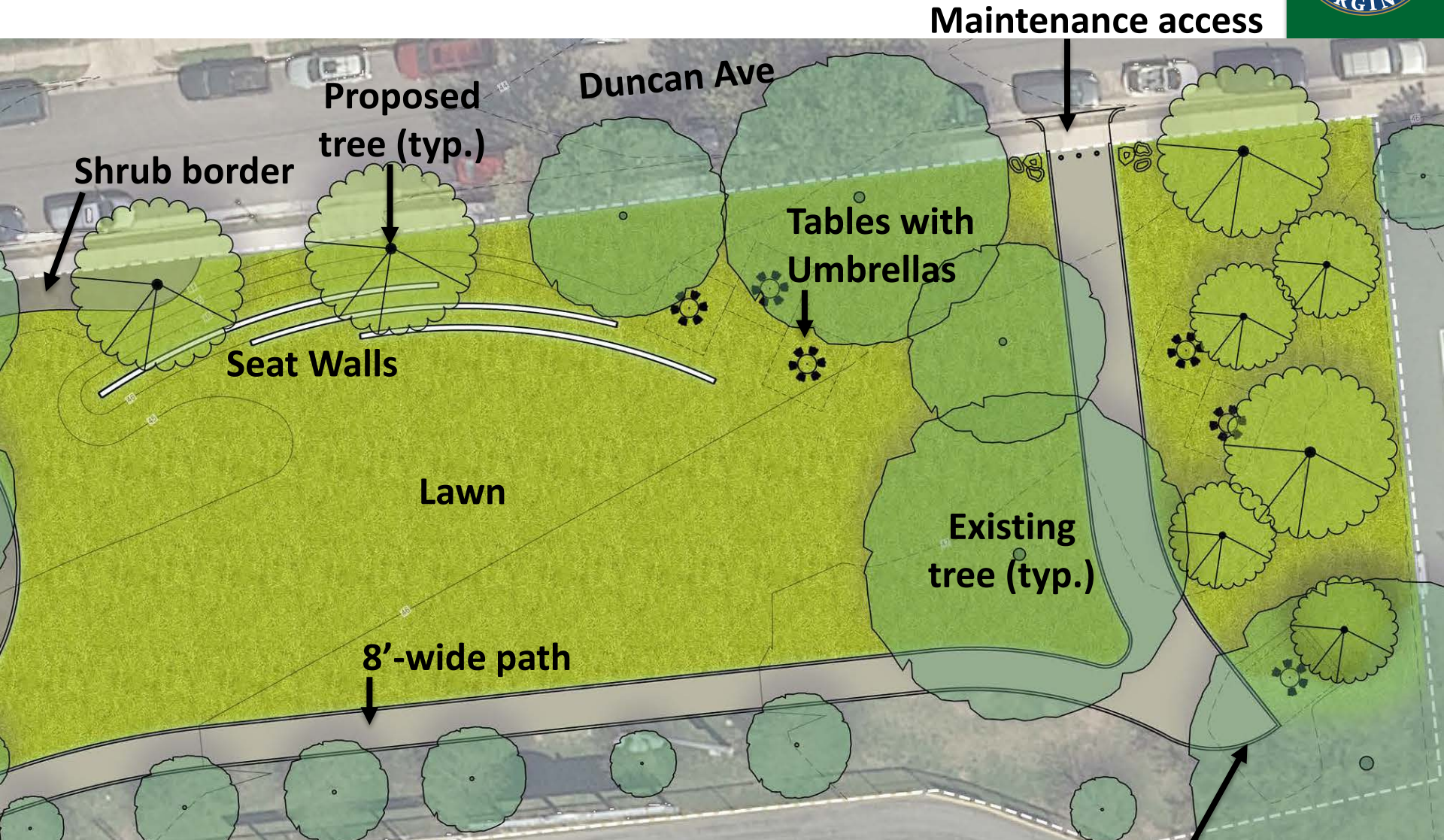
Accessible transition to and from existing stone dust path to permeable paver path
