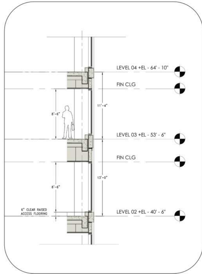
ENLARGED SECTION NTS.
