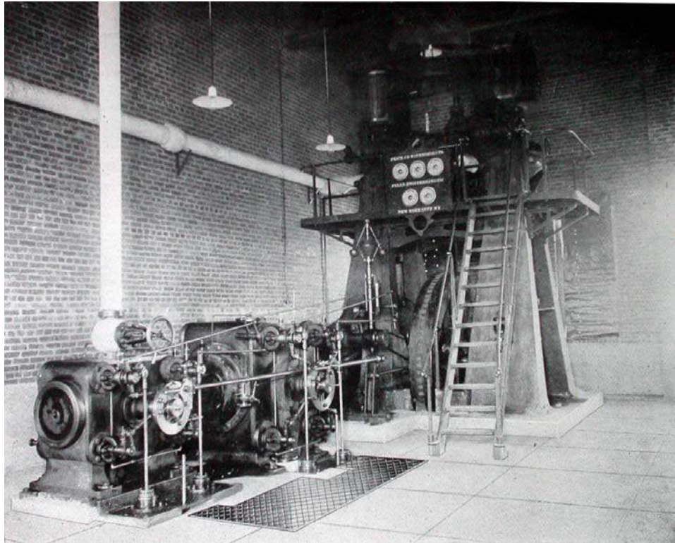
PLATE 16 Mutual Ice Company Frick Compressor; Adapted from Ice and Refrigeration
