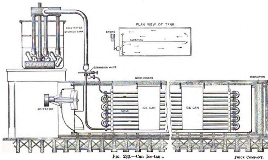
PLATE 3 Typical Can Ice Plant; Adapted from Lorenz 1905
