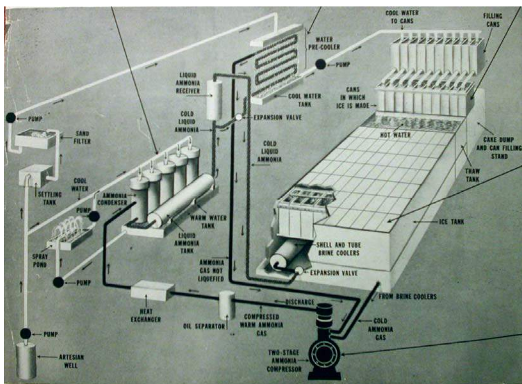
PLATE 25 Mutual Ice Company Process Flow Diagram; Adapted from Esso Oilways , 1946
