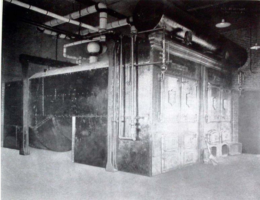
PLATE 18 Mutual Ice Company Boilers; Adapted From Ice And Refrigeration ; 1913
