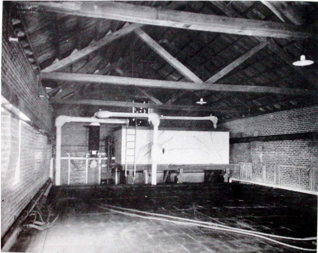
PLATE 14 Mutual Ice Company Freezing Room; Adapted from Ice and Refrigeration , 1913
