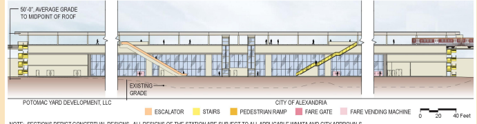
Alternative D-D' Longitudinal Section - View East
