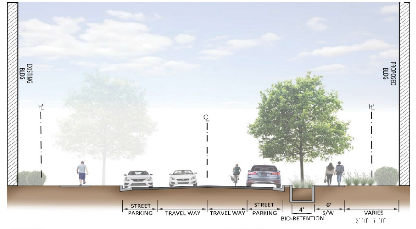
PROPOSED "NORTH ROYAL STREET" TYPICAL SECTION C - C1
