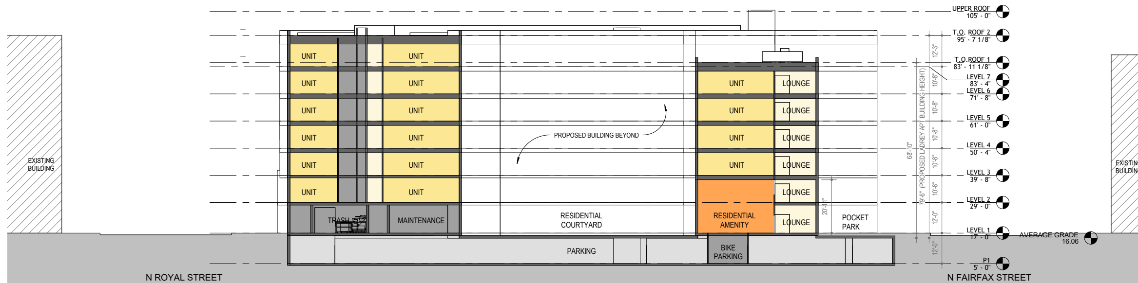
SECTION B-B
