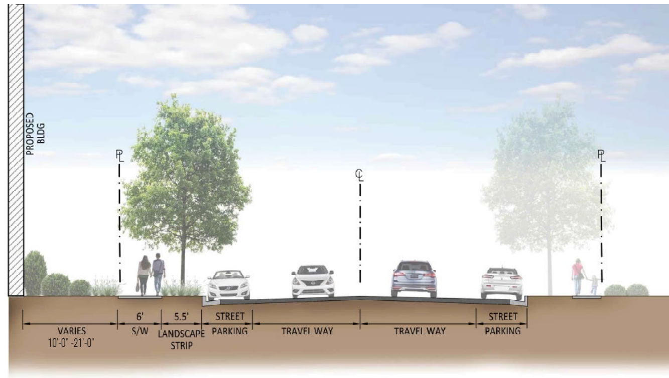
PROPOSED "WYTHE STREET" TYPICAL SECTION A - A1
