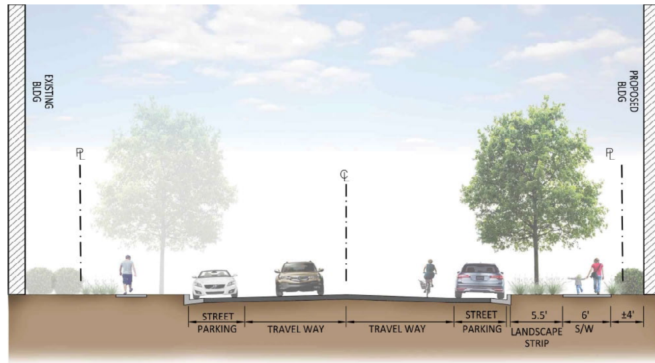
PROPOSED "PENDLETON STREET" TYPICAL SECTION B - B1
